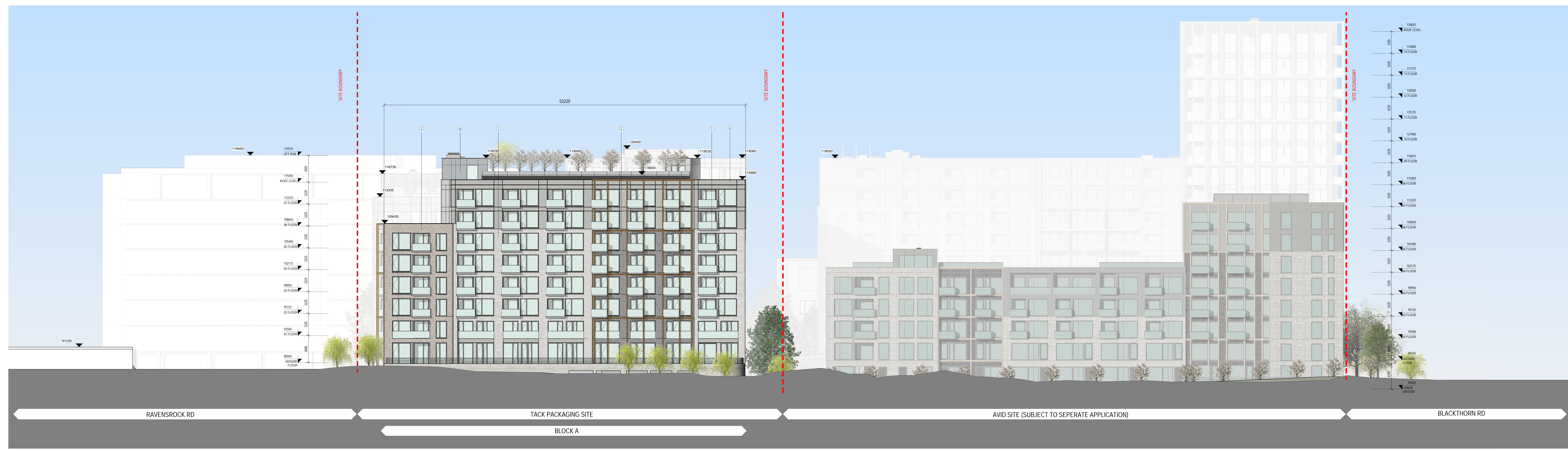
② PROPOSED SOUTH WEST CONTEXTUAL ELEVATION Scale: 1 : 200
